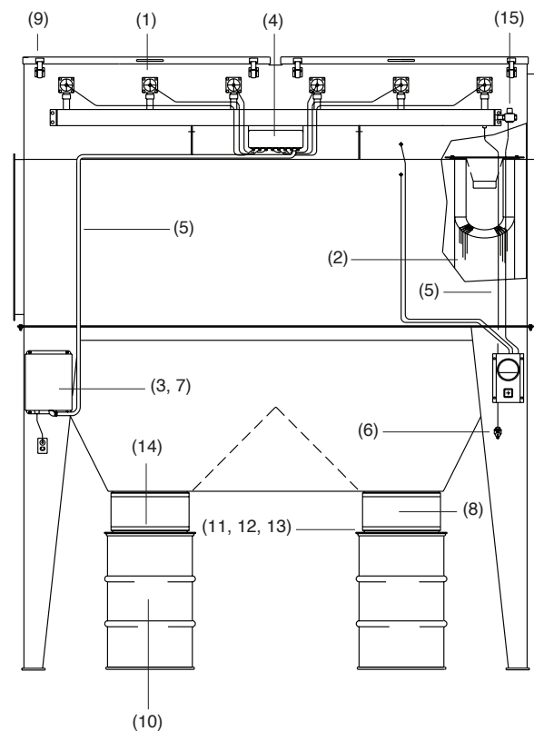
RPH-6 Reverse-Pulse Dust Collector
