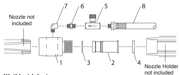
Wetblast Injector Nozzle Adaptor Assemblies
